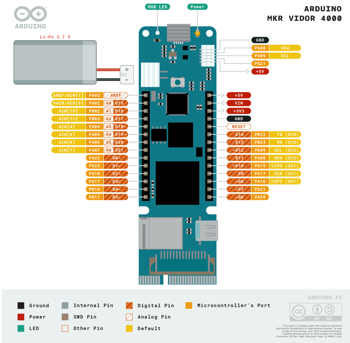
Figure 1. MKR Vidor basic pinout
