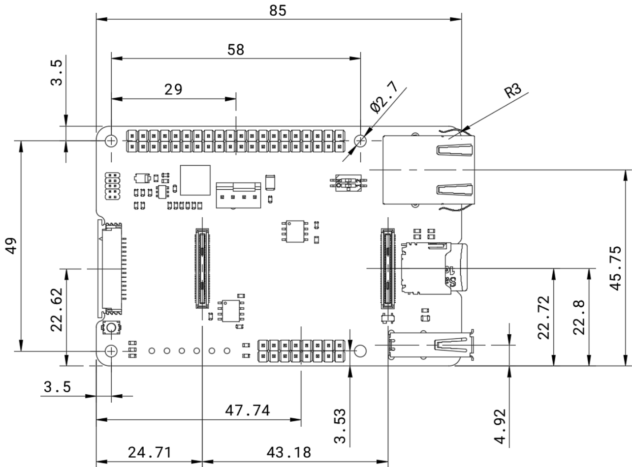
Figure 16. Portenta Hat Carrier board dimensions (in mm)
